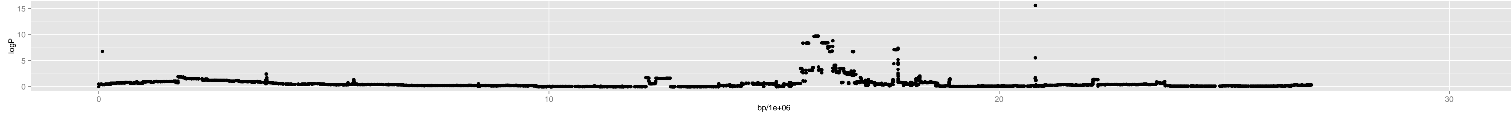
Chromosome 5 – 1_can.0_22842788_5_1
