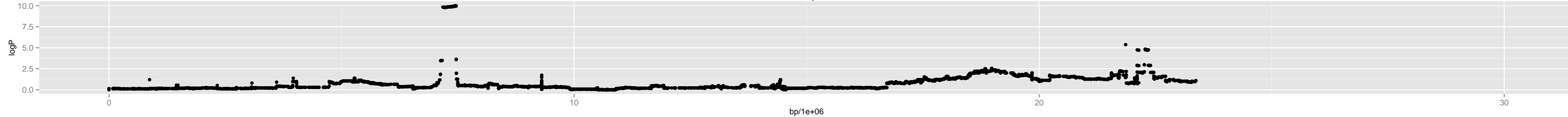
Chromosome 3 – 1_oy.0_11026223_7_2
