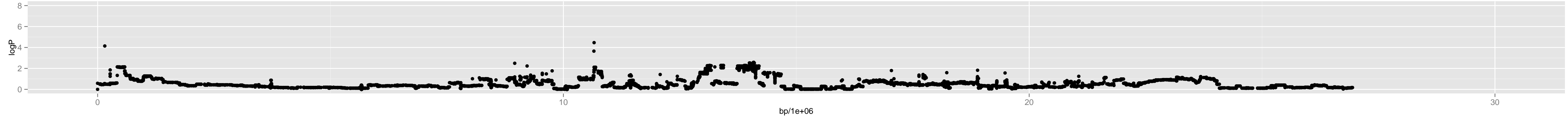
Chromosome 5 – 1_tsu.0_5470498_8_3
