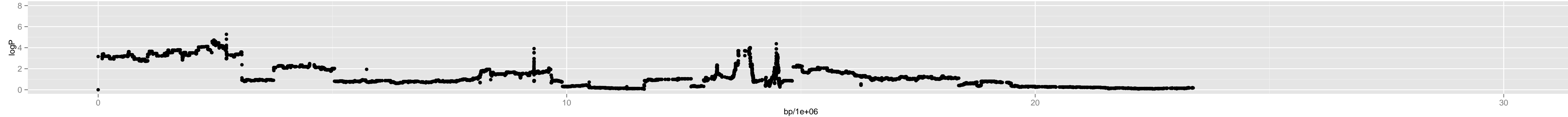
Chromosome 3 – 2_ct.1_9879_6_2
