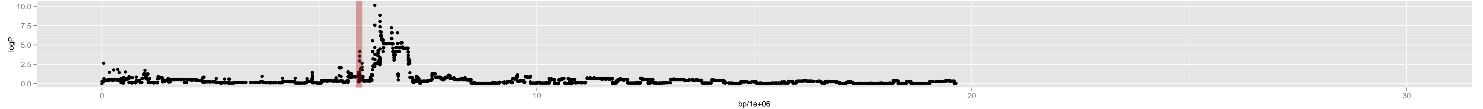
Chromosome 2 – 2_mt.0_5913037_5_1
