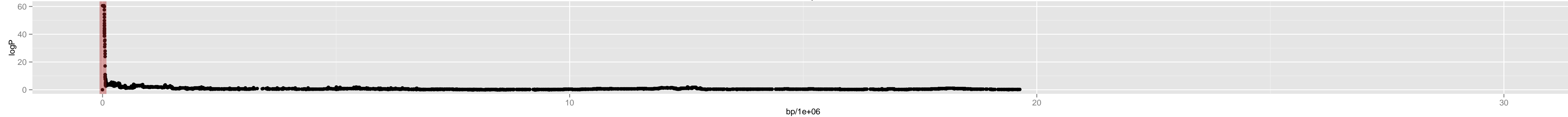
Chromosome 2 – 2_po.0_9879_28_7
