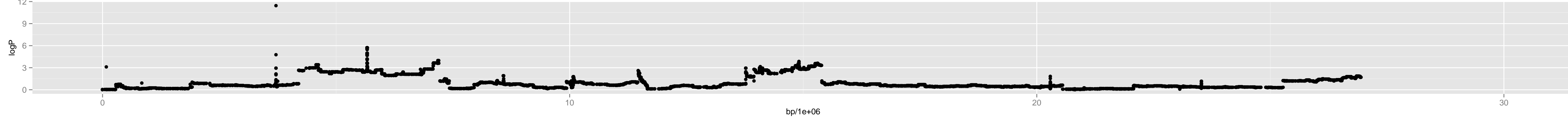
Chromosome 5 – 3_ct.1_14520257_7_4
