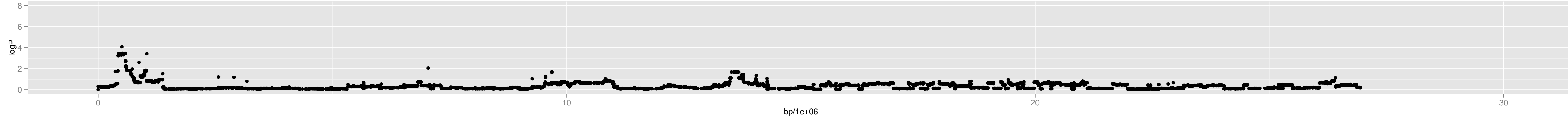
Chromosome 5 – 3_no.0_13551447_5_5
