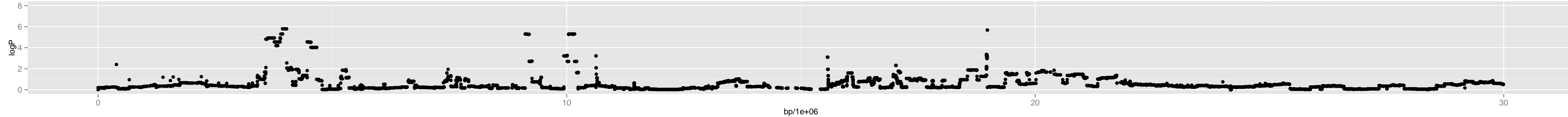
Chromosome 1 – 3_no.0_13551447_5_5
