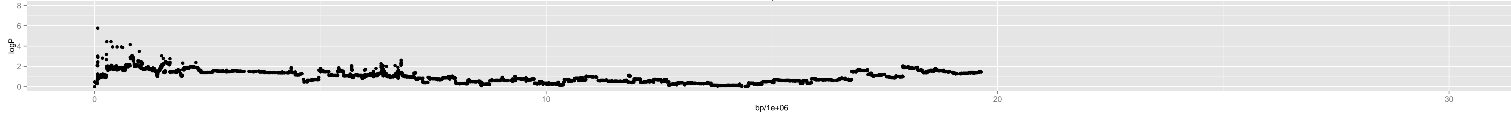
Chromosome 2 – 3_oy.0_13554998_13_10
