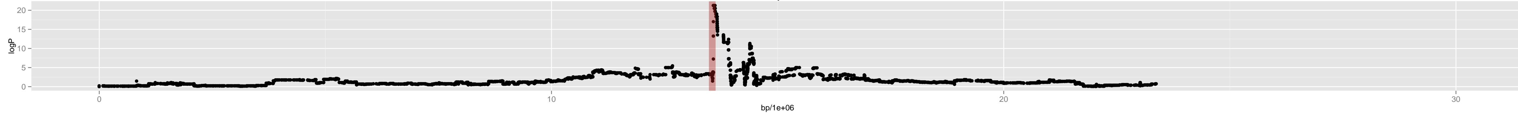
Chromosome 3 – 3_oy.0_13554998_13_10
