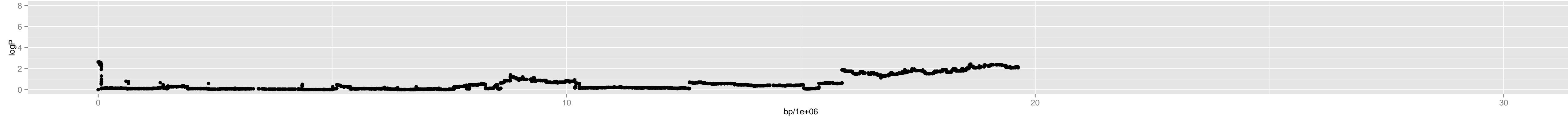
Chromosome 2 – 3_rsch.4_13960094_5_5
