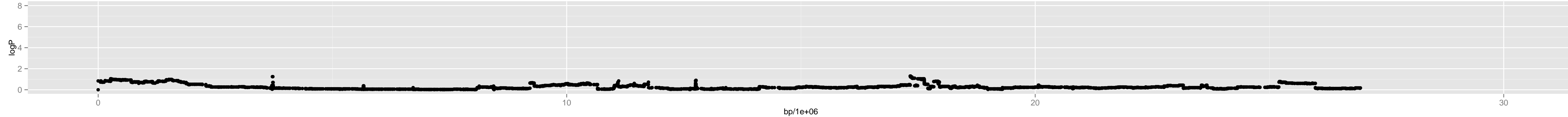
Chromosome 5 – 3_rsch.4_13960094_5_5
