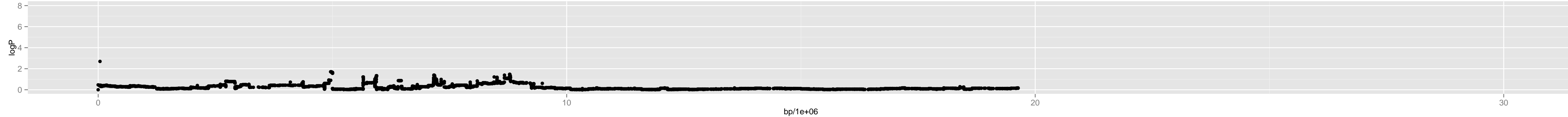
Chromosome 2 – 3_tsu.0_14274965_11_10
