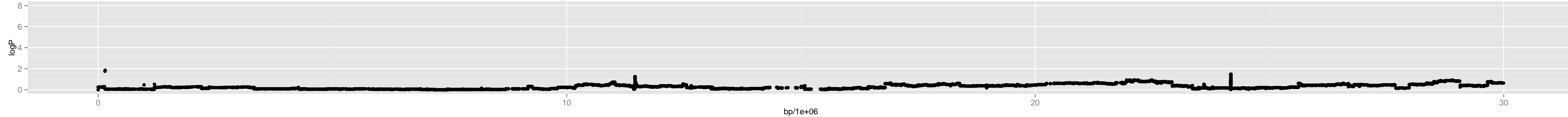
Chromosome 1 – 3_tsu.0_14274965_11_10
