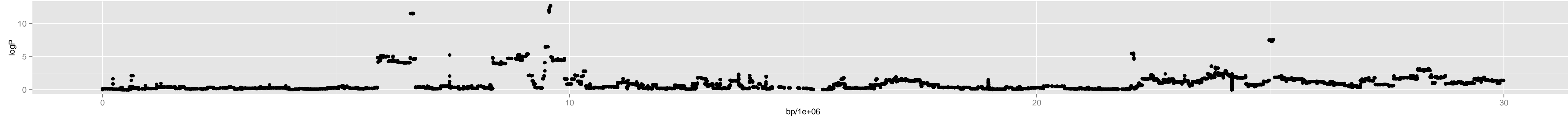
Chromosome 1 – 3_tsu.0_14374281_12_7
