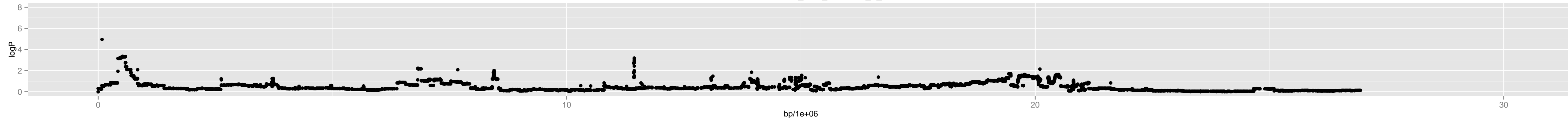
Chromosome 5 – 3_zu.0_9605779_6_2
