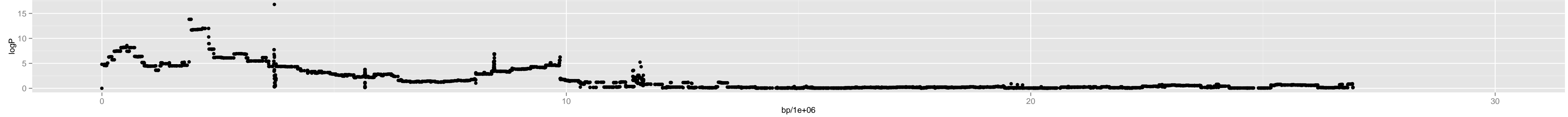
Chromosome 5 – 4_ct.1_4703112_6_1
