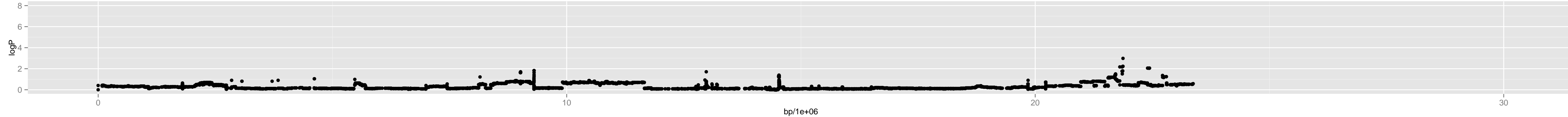
Chromosome 3 – 4_ct.1_4703112_6_1
