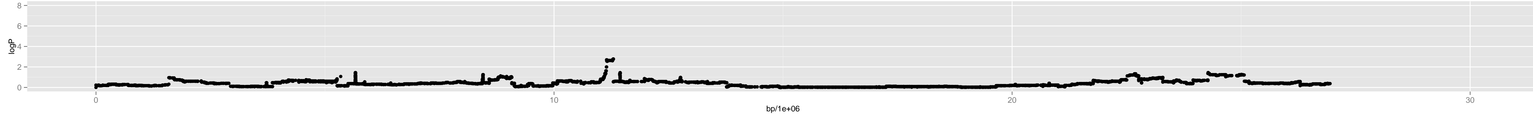
Chromosome 5 – 4_edi.0_4207240_8_6
