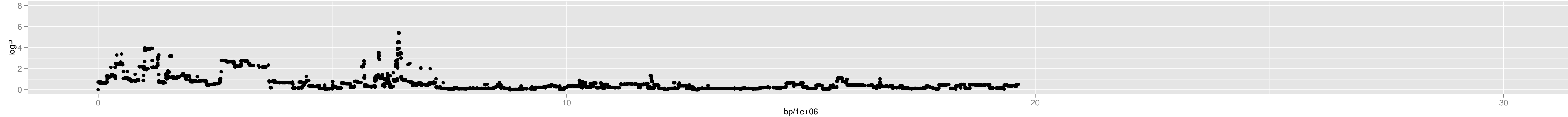
Chromosome 2 – 4_edi.0_4573507_9_6
