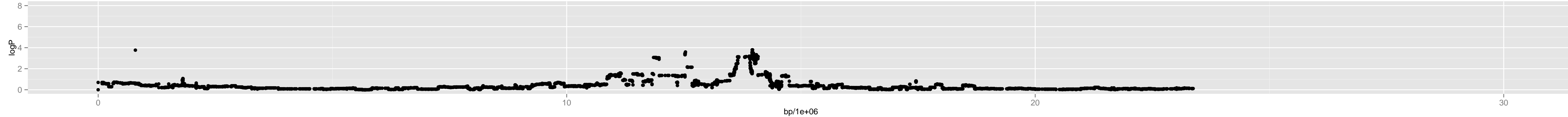
Chromosome 3 – 4_edi.0_4573507_9_6
