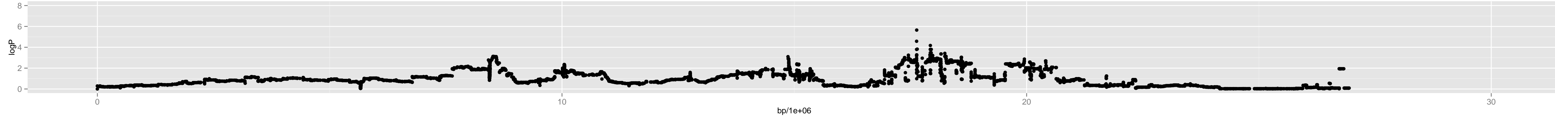
Chromosome 5 – 4_kn.0_714731_18_7
