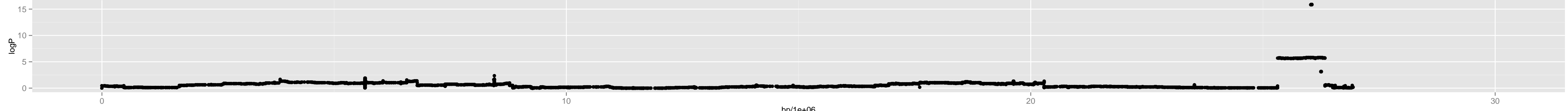
Chromosome 5 – 4_po.0_9436685_6_1
