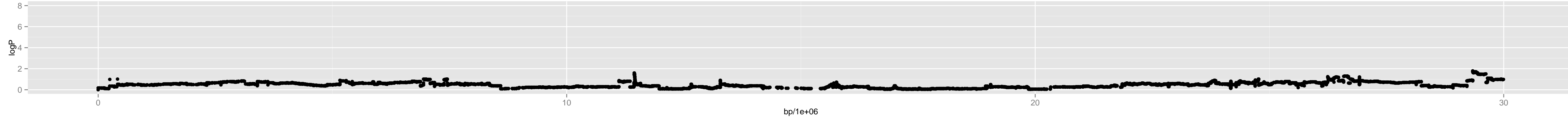
Chromosome 1 – 4_wu.0_6907428_12_2
