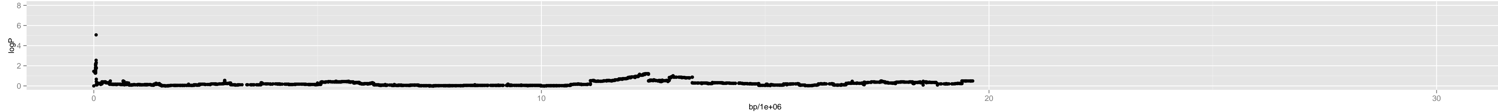
Chromosome 2 - 4_wu.0_6907428_12_2
