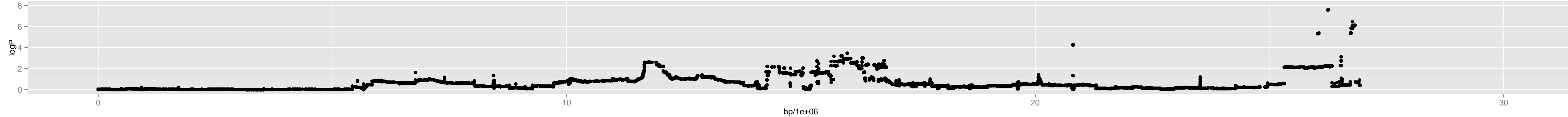
Chromosome 5 – 4_wu.0_6907428_12_2
