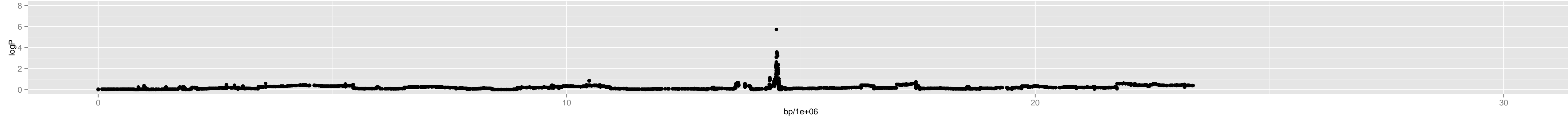
Chromosome 3 – 4_wu.0_6907428_12_2
