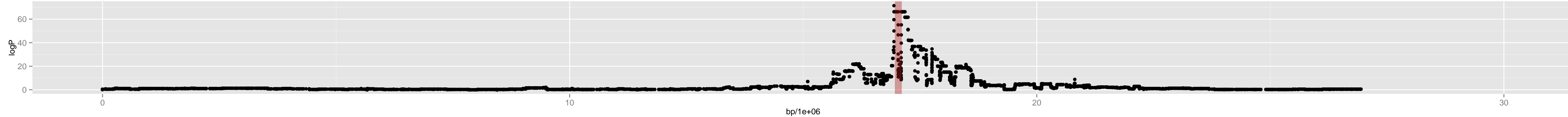
Chromosome 5 – 5_mt.0_17035475_14_5
