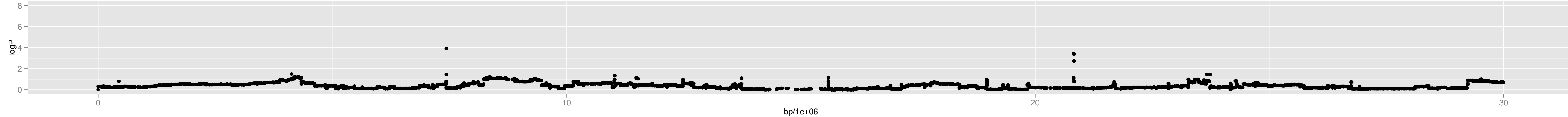
Chromosome 1 – 5_mt.0_17035475_14_5
