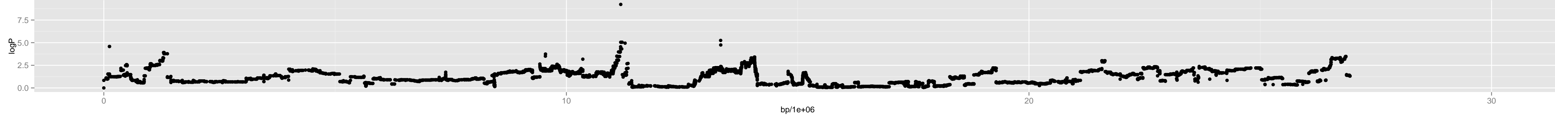
Chromosome 5 – 1_bur.0_18962190_10_4
