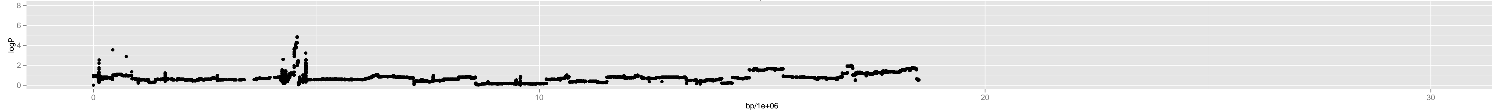
Chromosome 4 – 1_po.0_15584330_10_7
