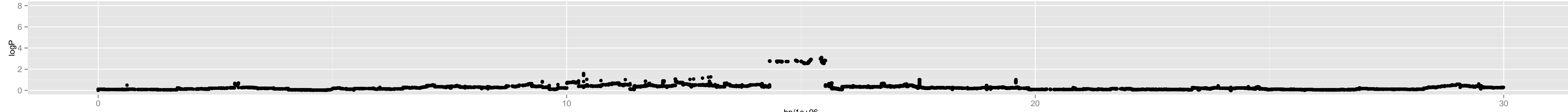
Chromosome 1 – 2_ler.0_5928579_11_11
