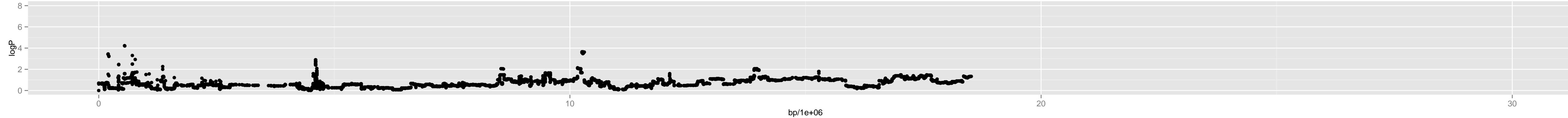
Chromosome 4 – 3_hi.0_14246685_18_2
