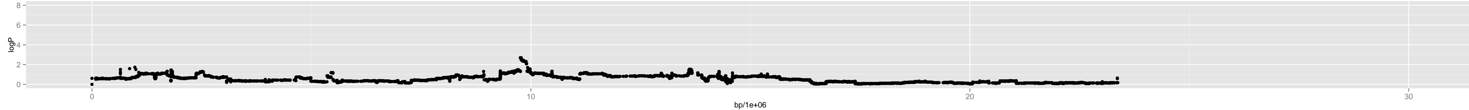
Chromosome 3 - 4_bur.0_4699956_12_8
