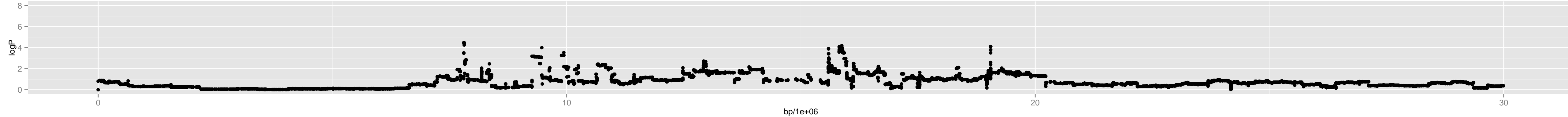
Chromosome 1 - 4_bur.0_4699956_12_8
