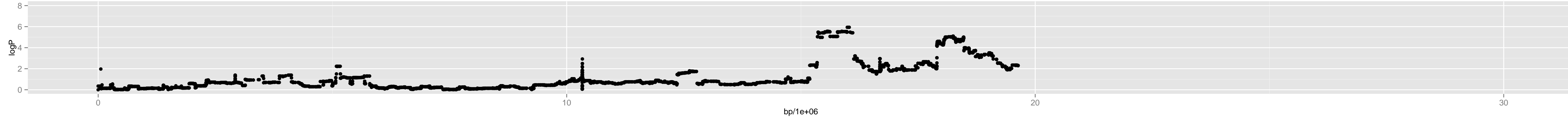
Chromosome 2 – 4_sf.2_4504329_11_7
