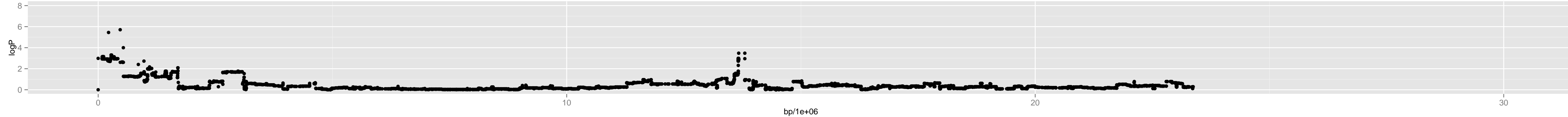
Chromosome 3 – 4_wu.0_4550735_12_9
