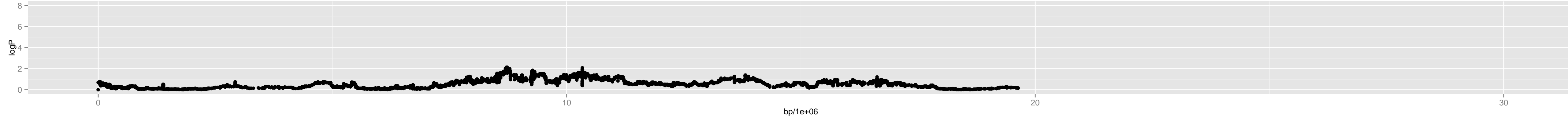
Chromosome 2 – Chr1_11000000
