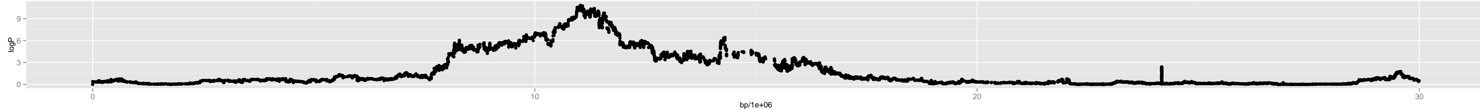
Chromosome 1 – Chr1_11000000
