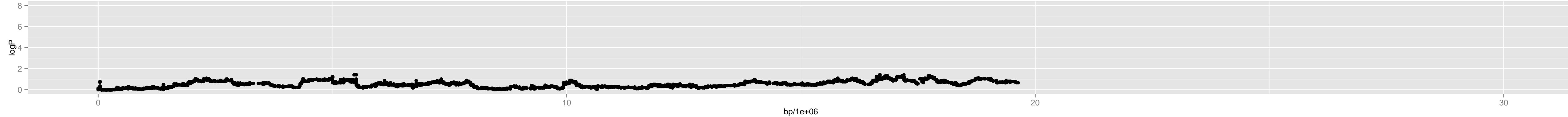
Chromosome 2 – Chr1_14900000
