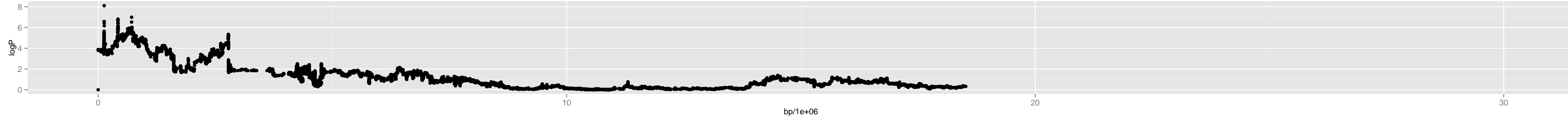
Chromosome 4 – Chr1_19400000
