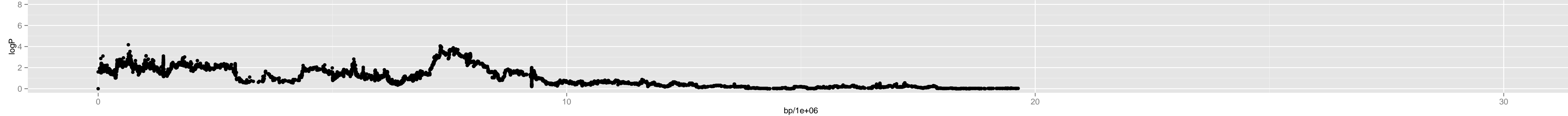
Chromosome 2 – Chr1_19400000
