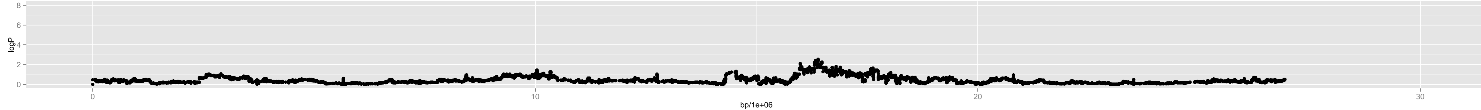
Chromosome 5 – Chr1_23600000
