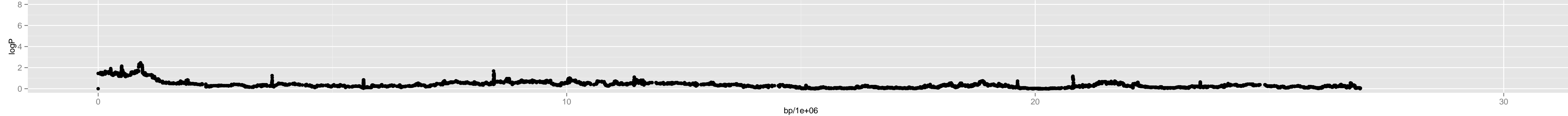
Chromosome 5 – Chr1_24800000
