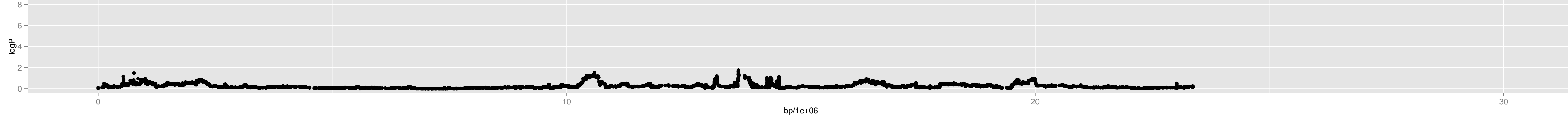
Chromosome 3 – Chr1_24800000
