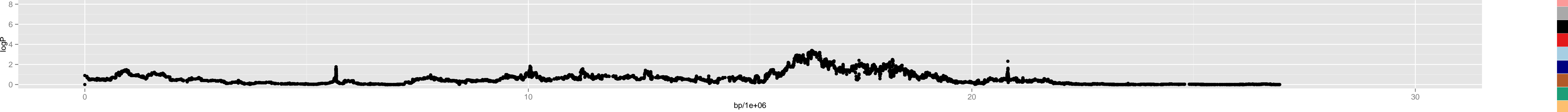
Chromosome 5 – Chr2_11200000
