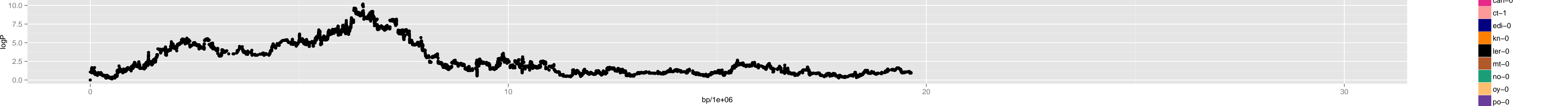
Chromosome 2 – Chr2_6300000
