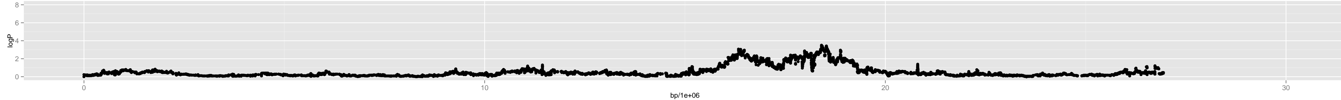
Chromosome 5 – Chr2_7900000
