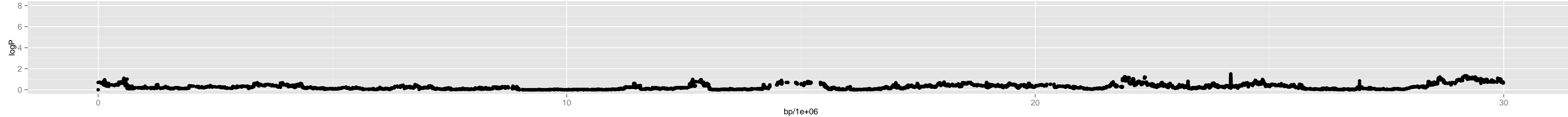
Chromosome 1 – Chr2_7900000
