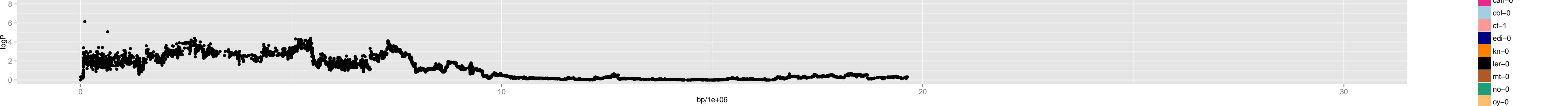
Chromosome 2 – Chr3_100000
