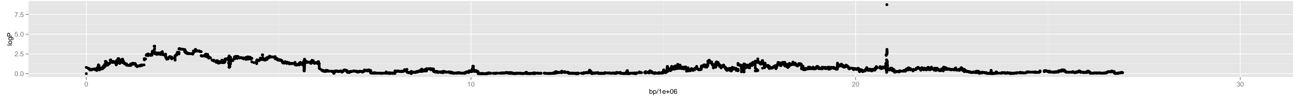
Chromosome 5 – Chr3_100000
