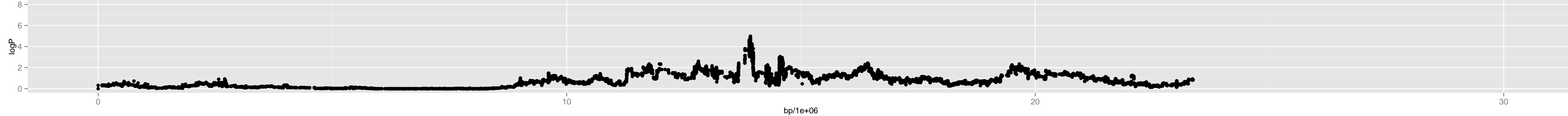
Chromosome 3 – Chr3_13300000
