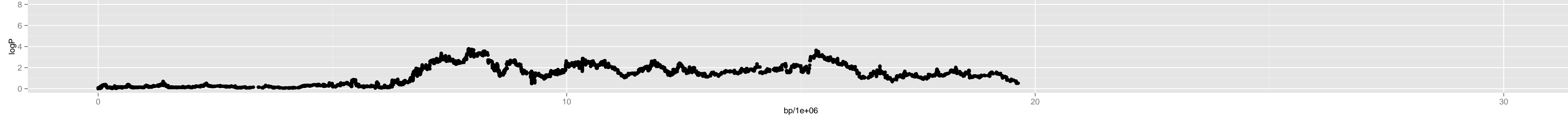
Chromosome 2 – Chr3_14300000
