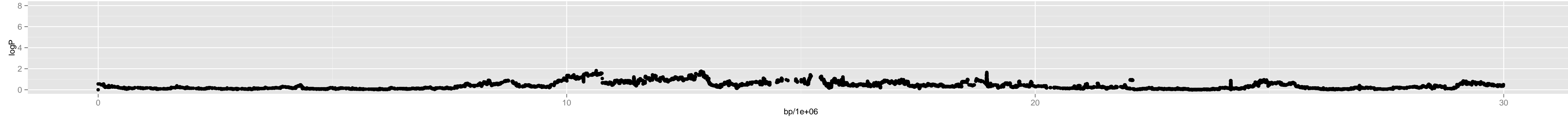
Chromosome 1 – Chr3_14700000
