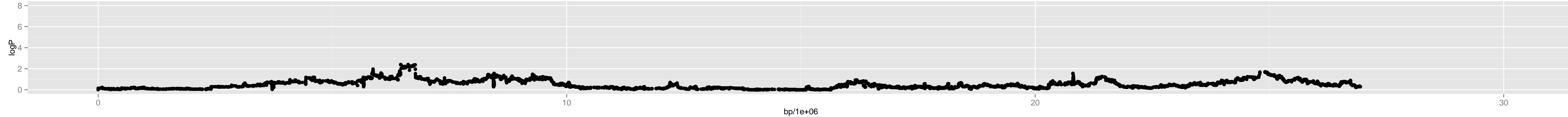
Chromosome 5 – Chr3_16000000
