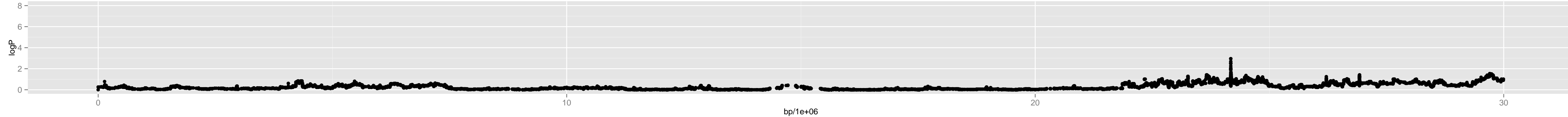
Chromosome 1 – Chr3_18700000
