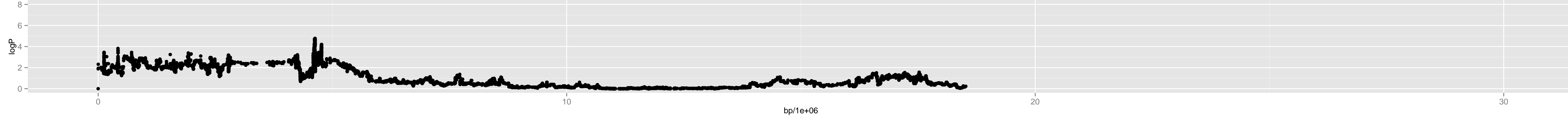
Chromosome 4 – Chr3_18700000
