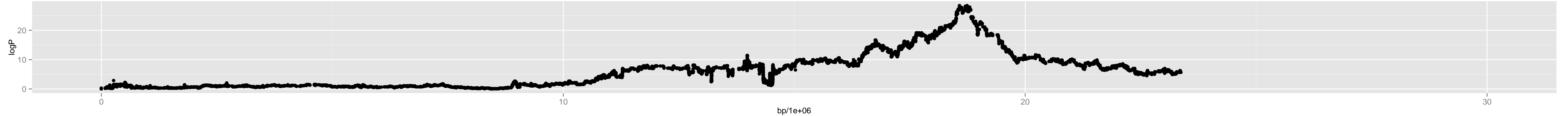
Chromosome 3 – Chr3_18700000
