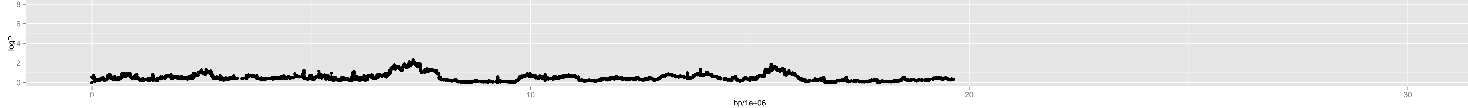
Chromosome 2 – Chr3_19500000
