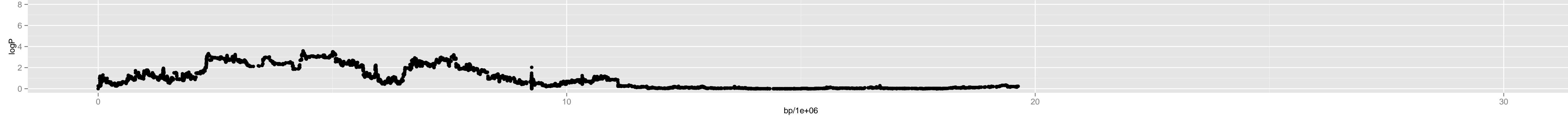
Chromosome 2 – Chr4_11600000
