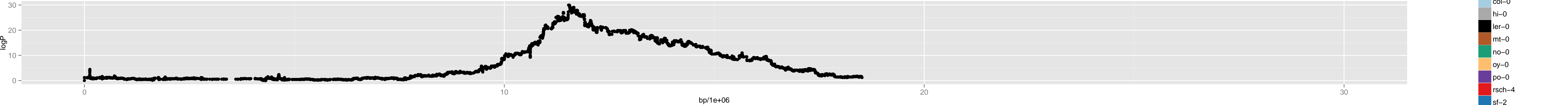
Chromosome 4 – Chr4_11600000
