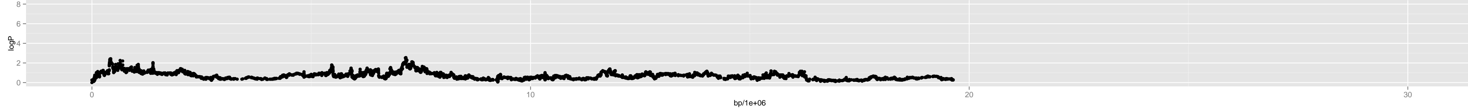
Chromosome 2 – Chr4_14200000
