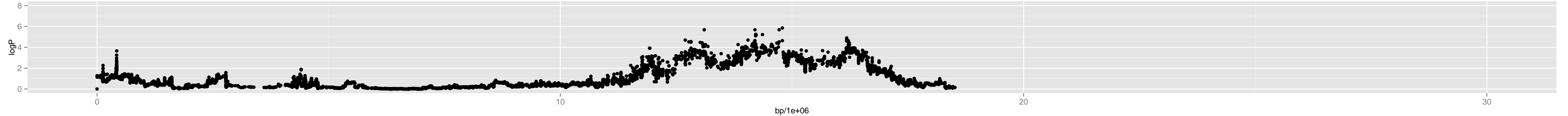
Chromosome 4 – Chr4_14200000
