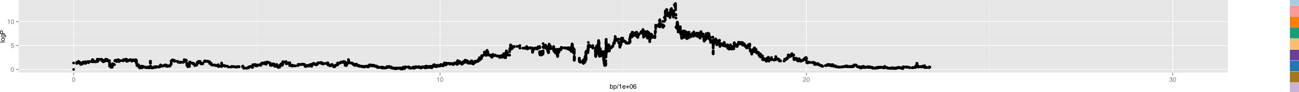
Chromosome 3 – Chr4_14200000
