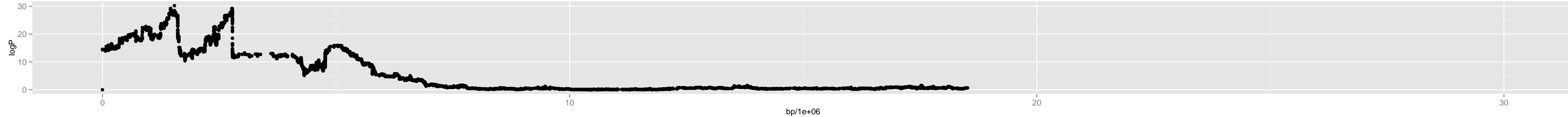
Chromosome 4 – Chr4_1500000
