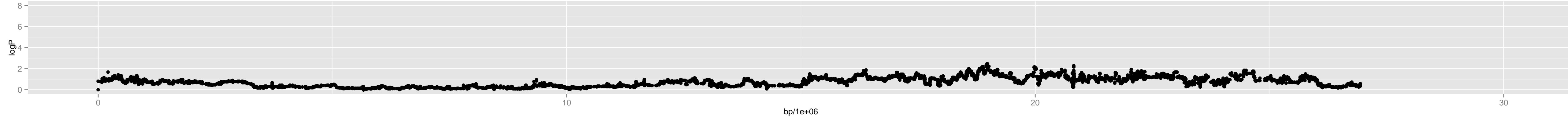
Chromosome 5 – Chr4_16200000
