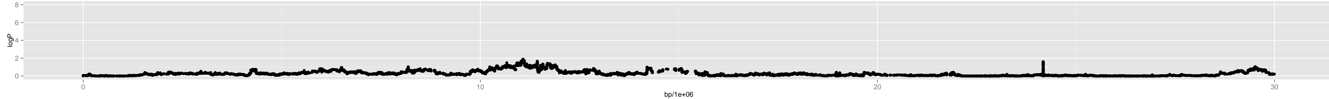
Chromosome 1 – Chr5_14700000
