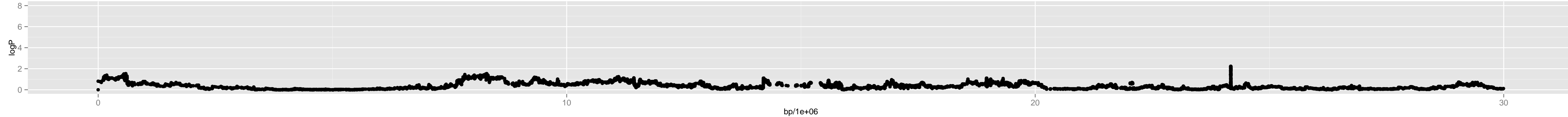
Chromosome 1 – Chr5_15800000
