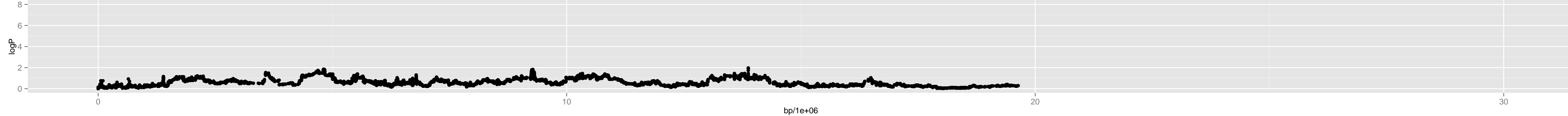
Chromosome 2 – Chr5_17300000
