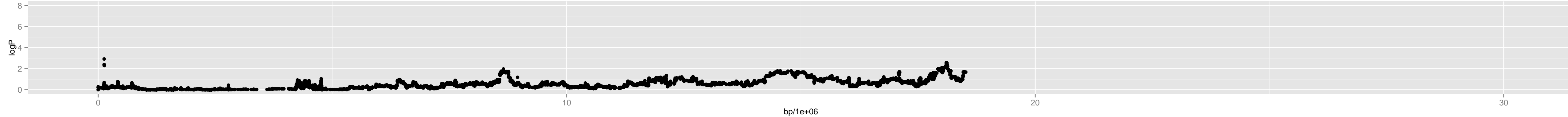
Chromosome 4 – Chr5_17300000
