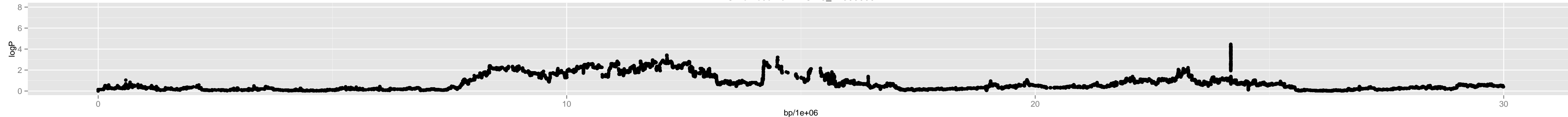
Chromosome 1 – Chr5_17300000
