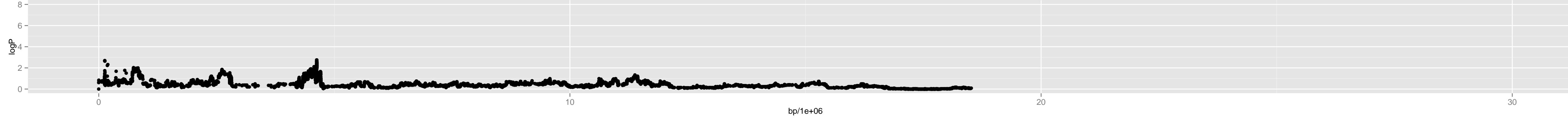
Chromosome 4 – Chr5_19500000
